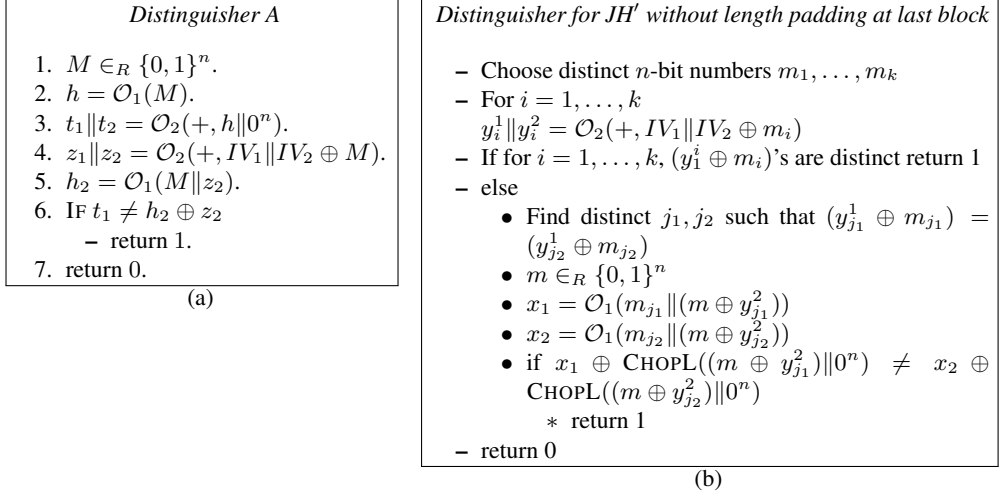
Fig. 6. 6(a): Distinguisher for JH- n without length padding, 6(b): Distinguisher for JH' without length padding
